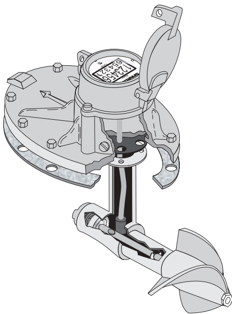
Figure 1 Principle of Operation
